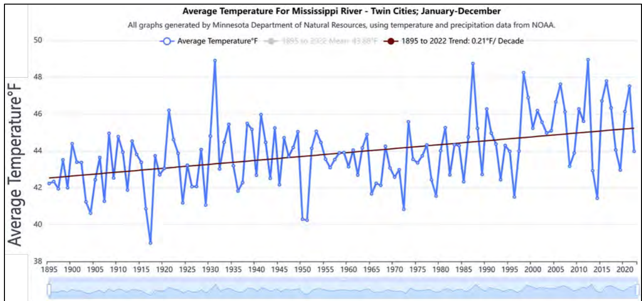
GRAPH 7-1 HISTORICAL TEMPERATURE TRENDS
