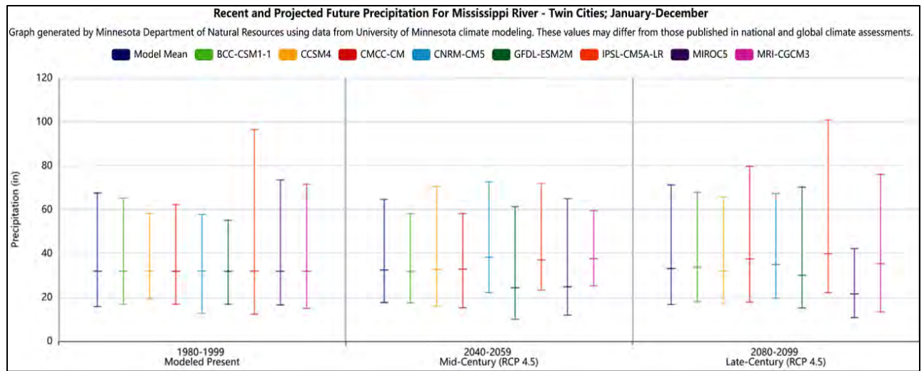
GRAPH 7-4 FUTURE PRECIPITATION TRENDS
